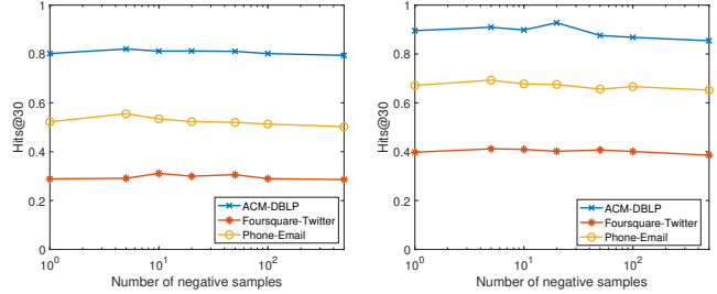
(a) 10% training data. (b) 20% training data.
