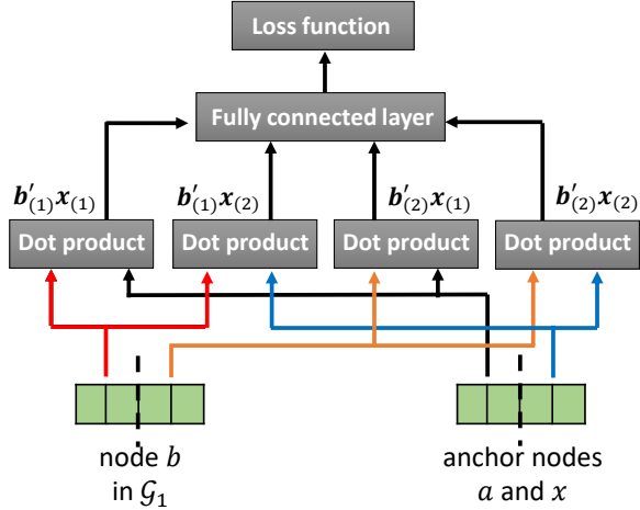
Figure 3: Illustration of embedding interactions.
