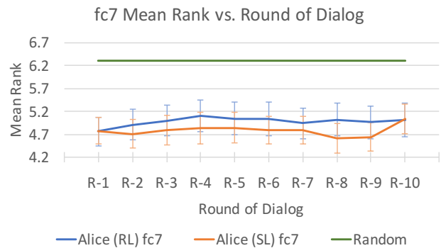
(b) ALICE SL and ALICE RL perform about the same, and clearly outperform a baseline model that randomly chooses an image. As described in Sec. 4.3, this is only a coarse estimate of the rank of the secret image after each round of dialog.
