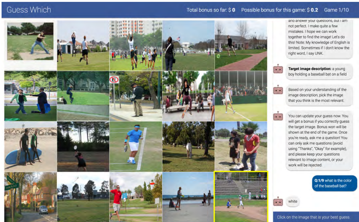
Figure 2: GuessWhich Interface: A user asks a question to ALICE in each round and ALICE responds with an answer. The user then selects an appropriate image which they think is the secret image after each round of conversation. At the end of the dialog, user successively clicks on their best guesses until they correctly identify the secret image.
