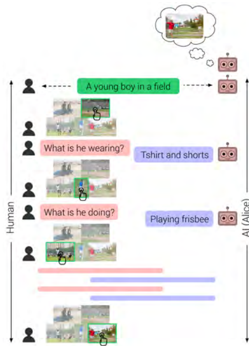
Figure 1: A human and an AI (a visual conversation agent called ALICE) play the proposed GuessWhich game. At the start of the game (top), ALICE is provided an image (shown above ALICE) which is unknown to the human. Both ALICE and the human are then provided a brief description of the image. The human then attempts to identify the secret image. In each subsequent round of dialog, the human asks a question about the unknown image, receives an answer from ALICE, and makes a best guess of the secret image from a fixed pool of images. After 9 rounds of dialog, the human makes consecutive guesses until the secret image is identified. The fewer guesses the human needs to identify the secret image, the better the human-AI team performance.
